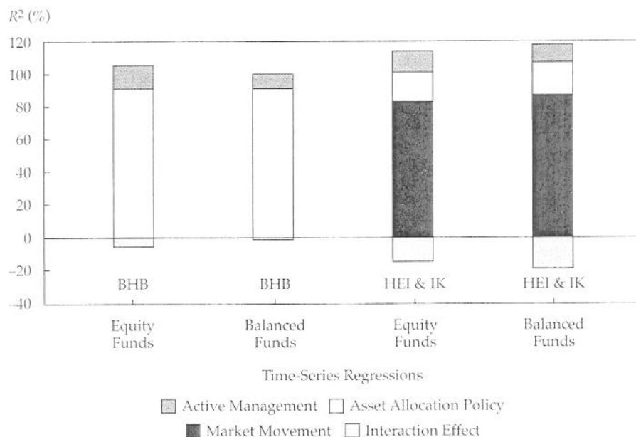
Figure 1. Decomposition of Time-Series Total Return Variations
